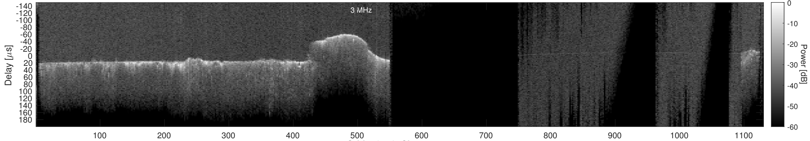
Orbit 13518, Cluttergram
