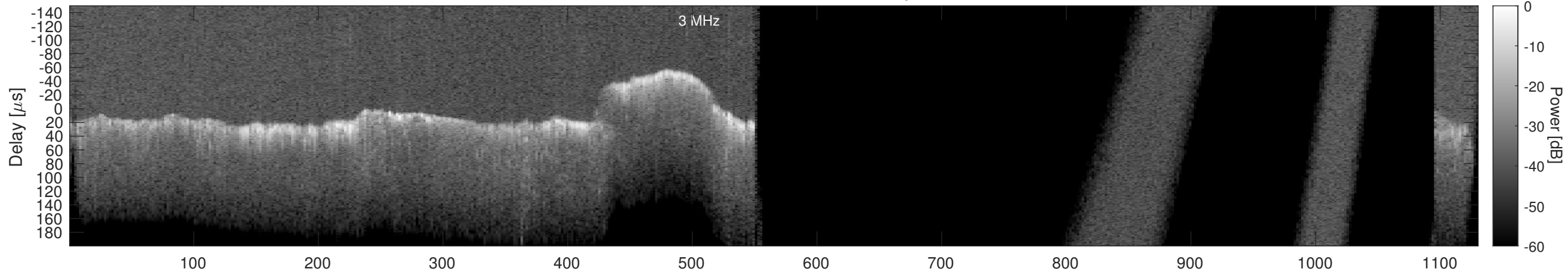
Orbit 13518, Window, Channel 2, Optimized
