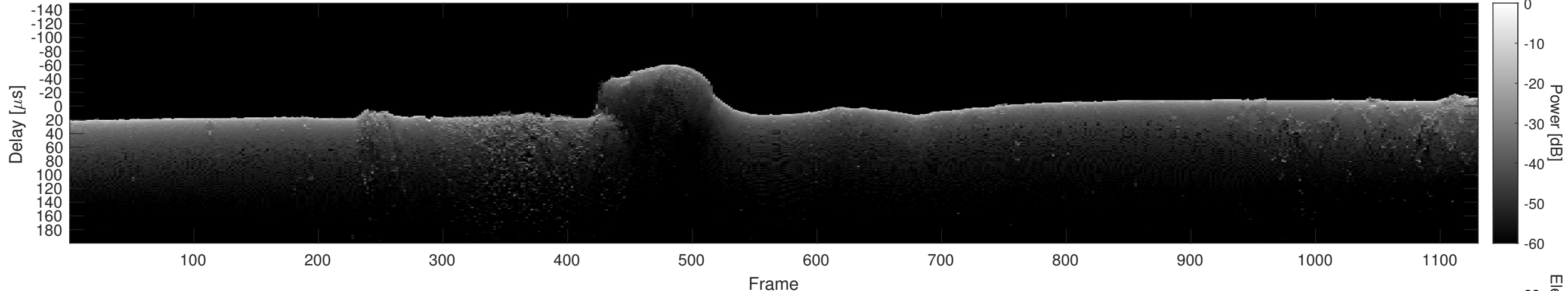
Orbit 13518, Cluttergram
