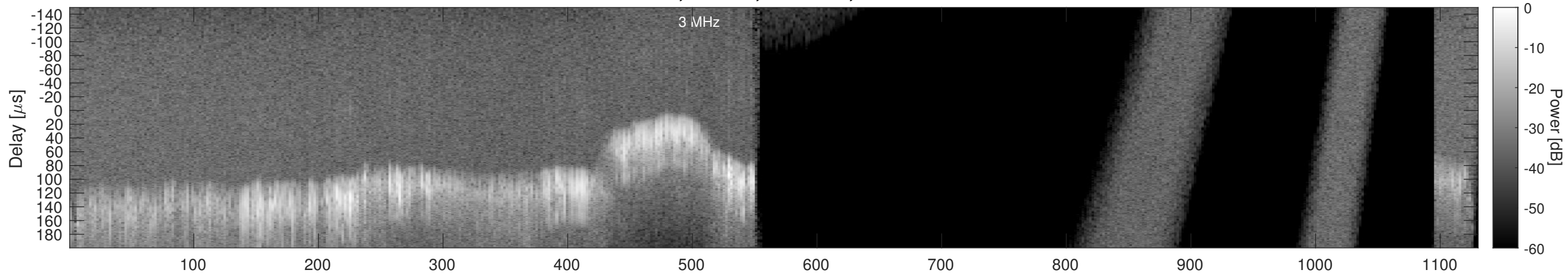
Orbit 13518, Window, Channel 2, Chapman
