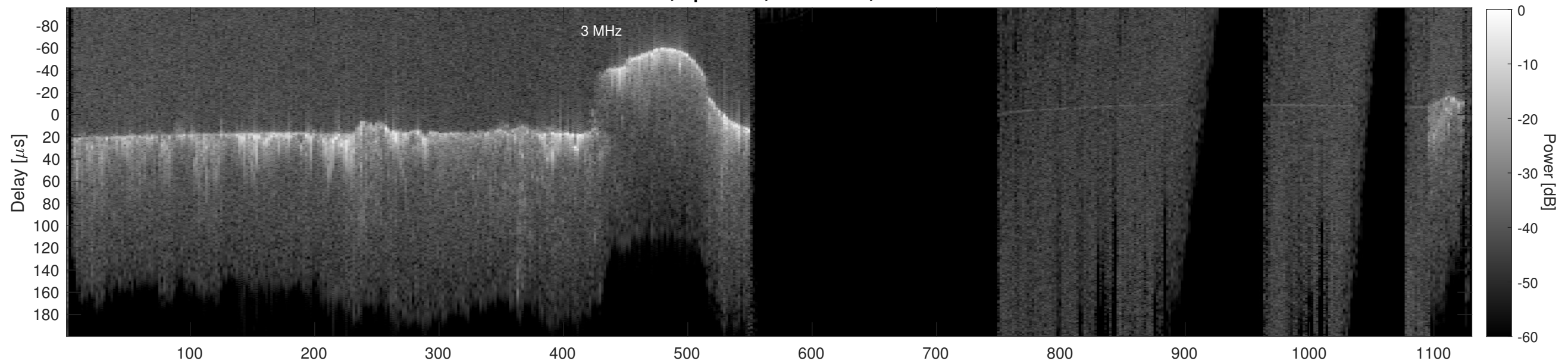
Orbit 13518, Cluttergram
