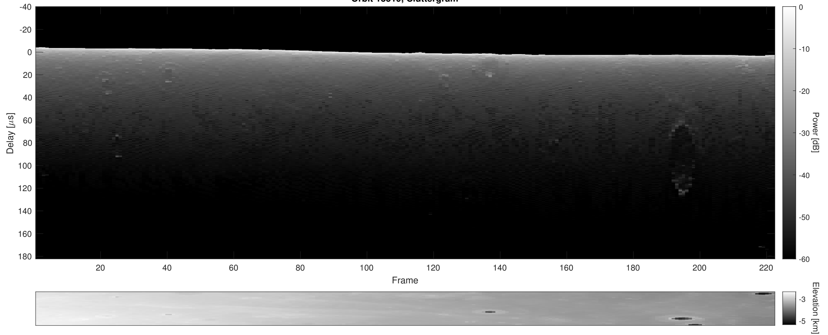
Orbit 13519, Cluttergram
