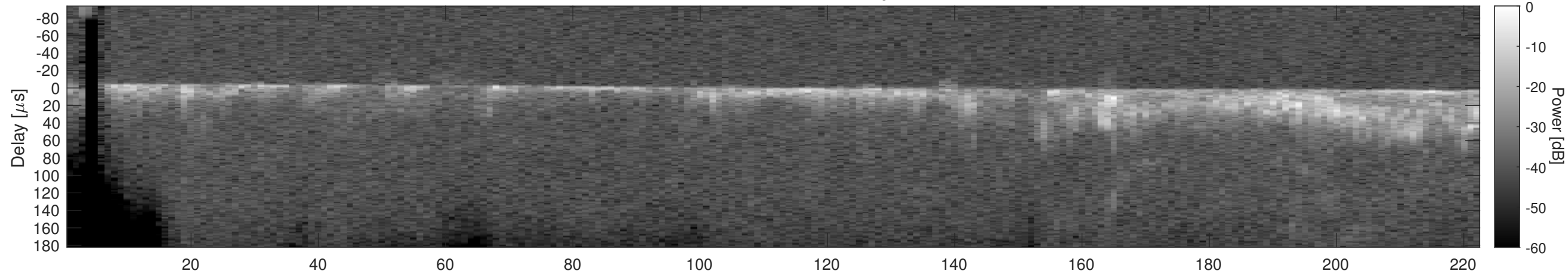
Orbit 13519, Cluttergram
