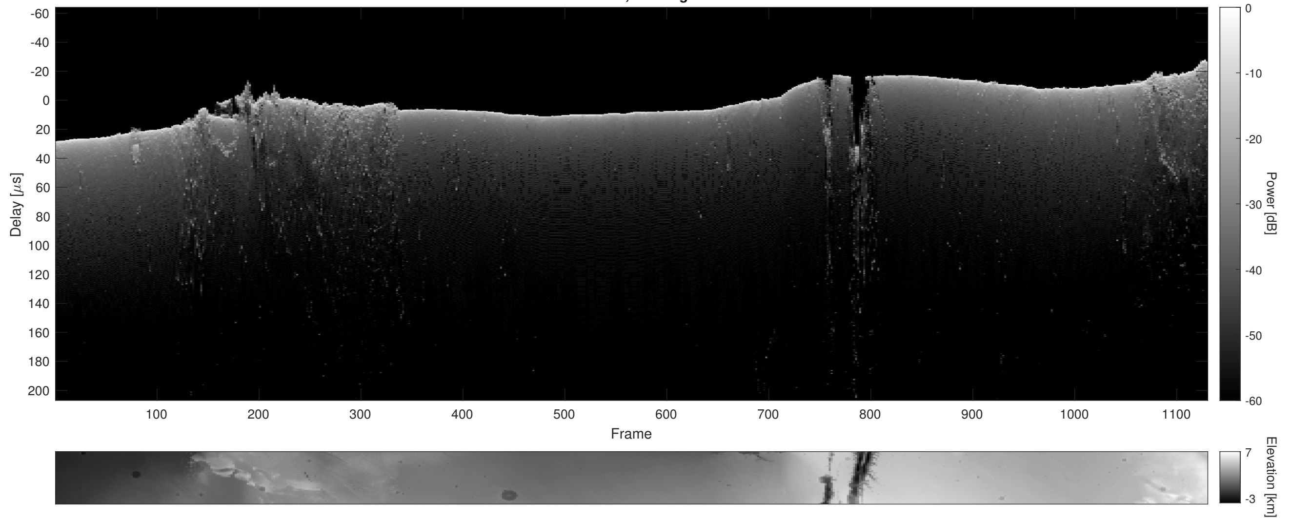
Orbit 13521, Cluttergram
