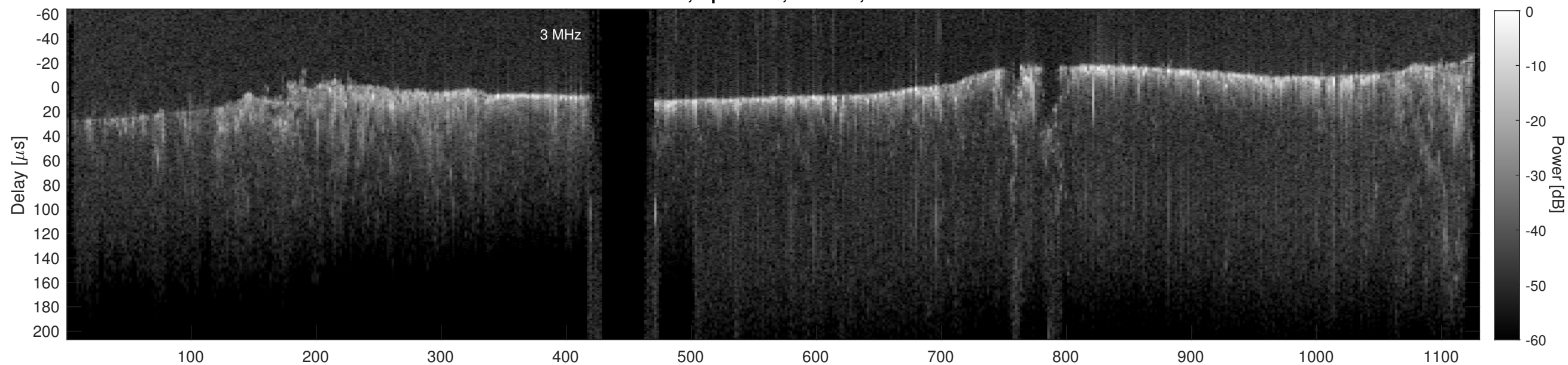
Orbit 13521, Cluttergram
