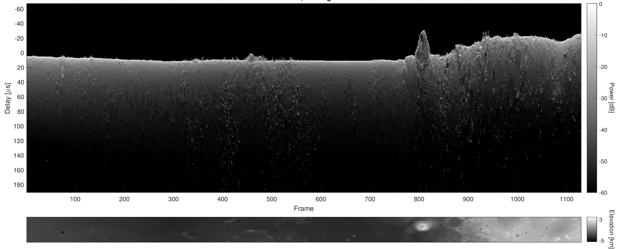
Orbit 13522, Cluttergram
