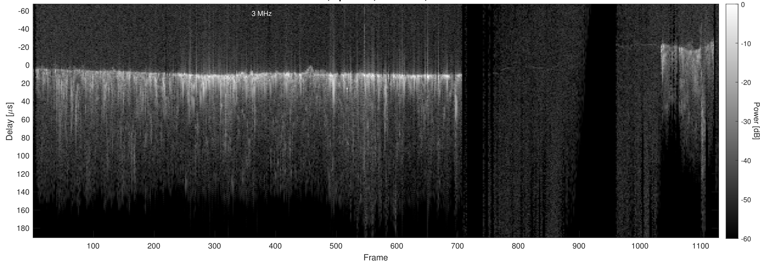
Orbit 13522, Optimized, No Window, Channel 2
