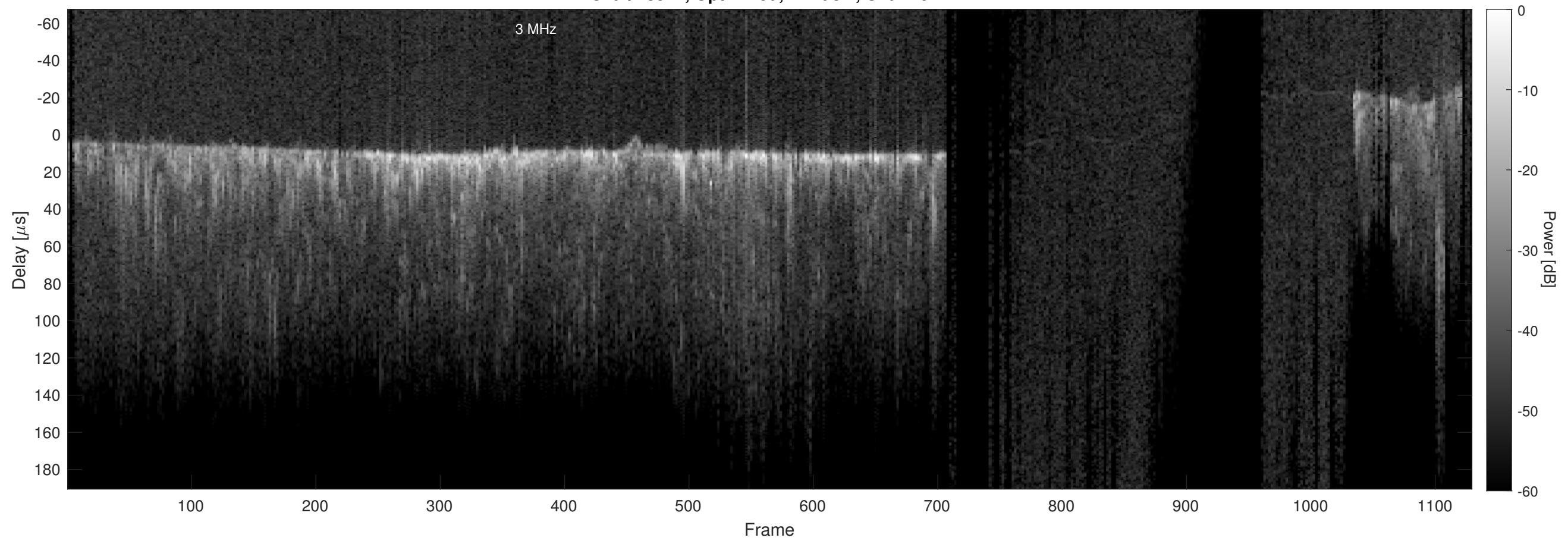
Orbit 13522, Optimized, Window, Channel 2
