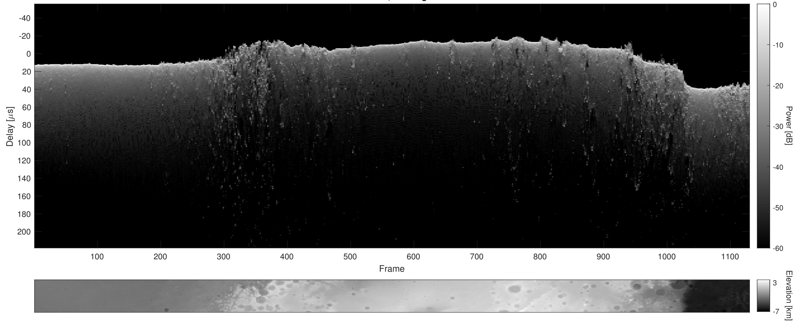
Orbit 13523, Cluttergram
