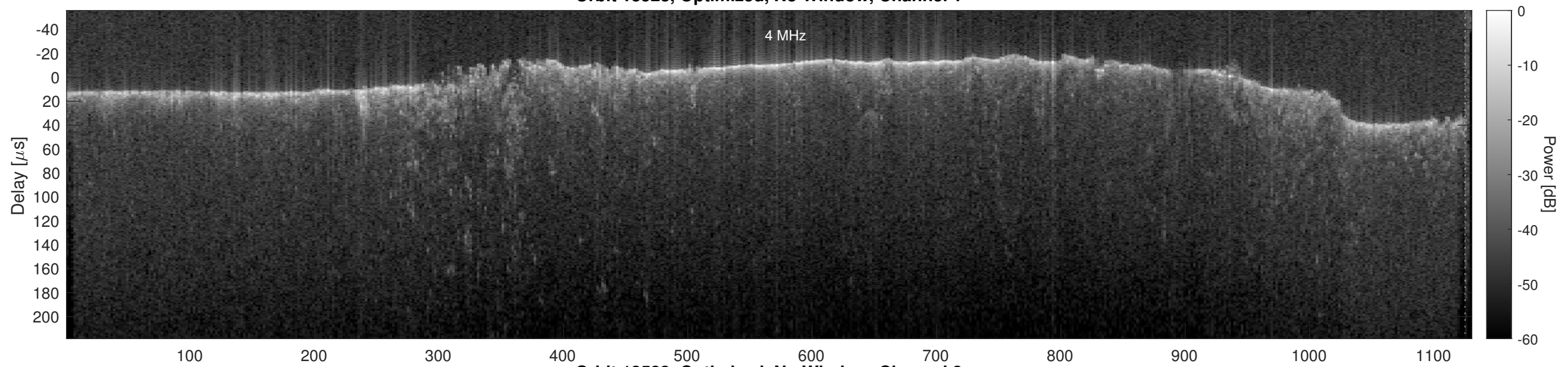
Orbit 13523, Optimized, No Window, Channel 2
