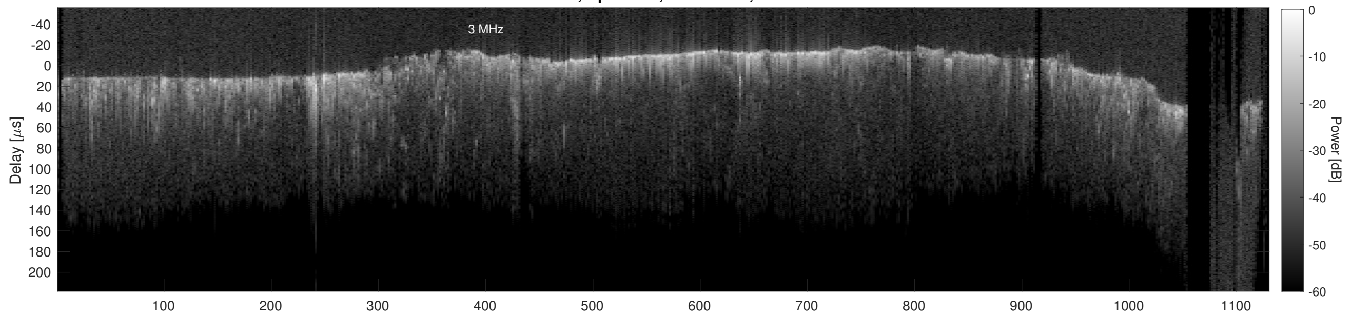
Orbit 13523, Cluttergram
