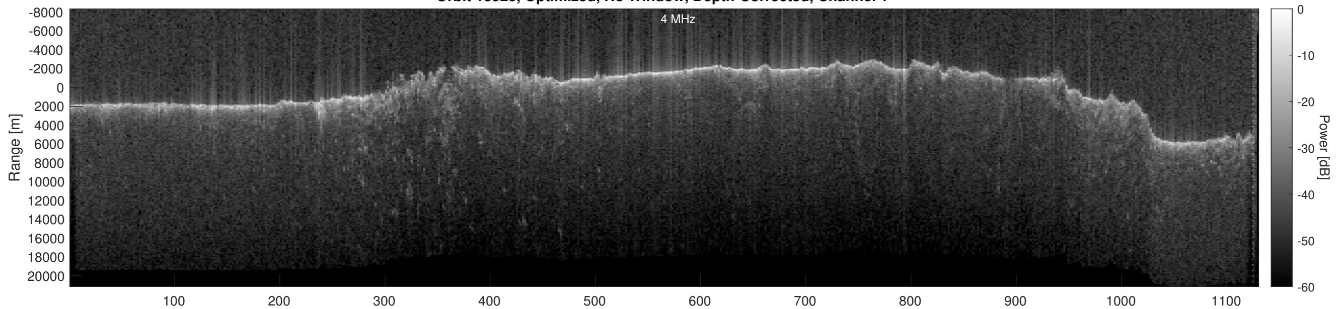
Orbit 13523, Optimized, No Window, Depth-Corrected, Channel 2
