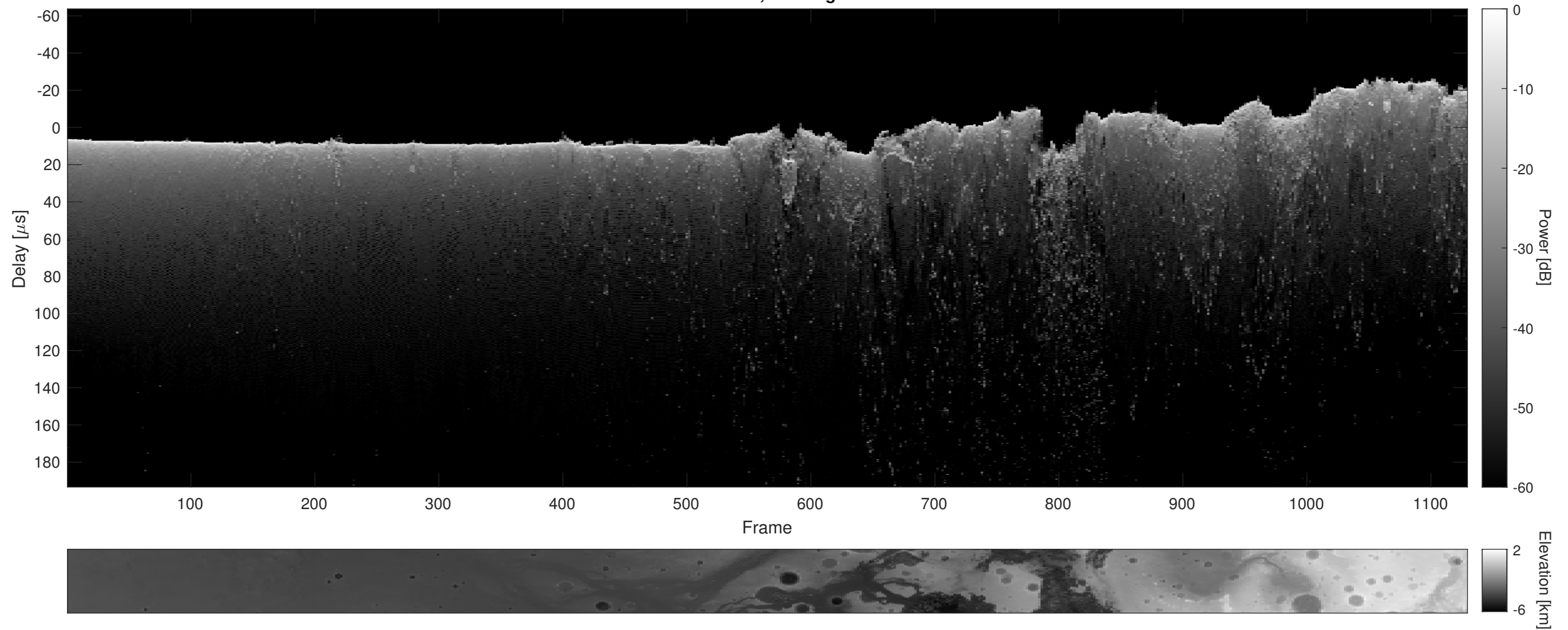
Orbit 13524, Cluttergram
