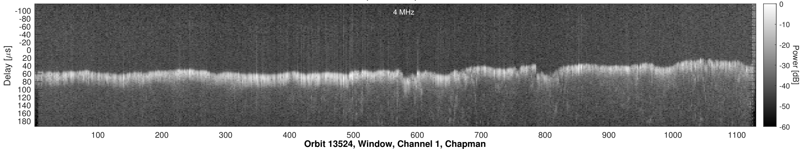
Orbit 13524, Channel 1, Uncorrected
