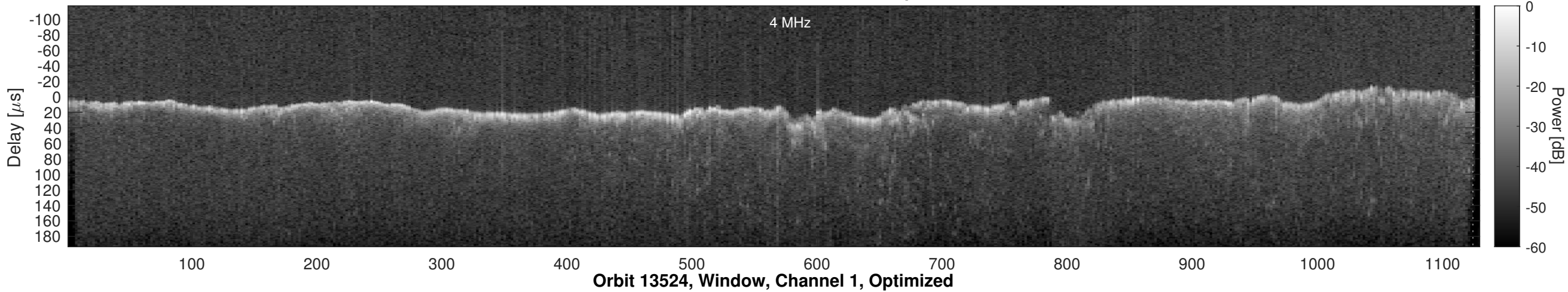
Orbit 13524, Window, Channel 1, Chapman
