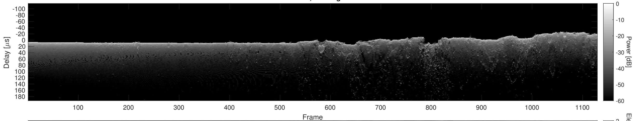
Orbit 13524, Cluttergram
