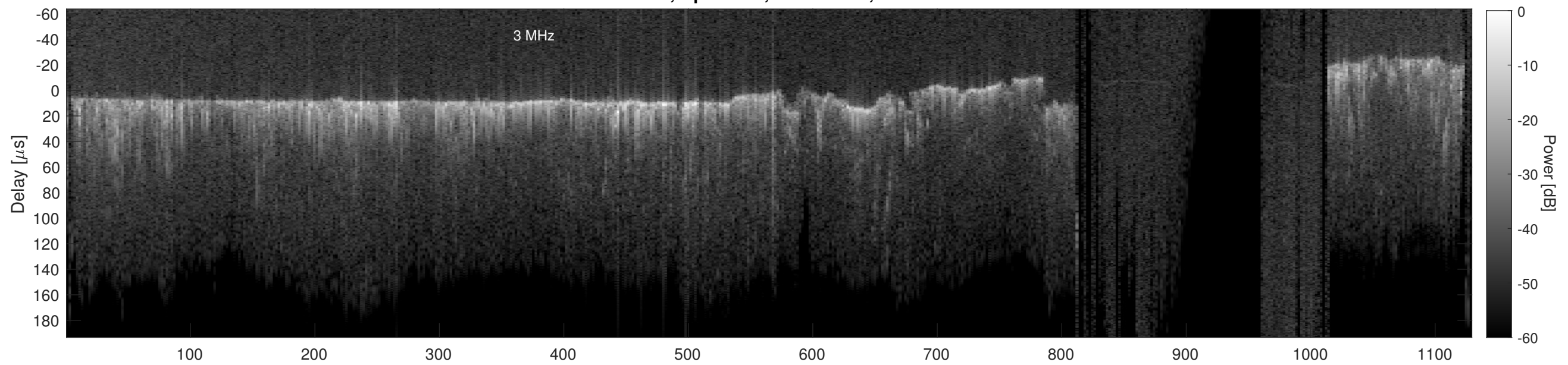
Orbit 13524, Cluttergram
