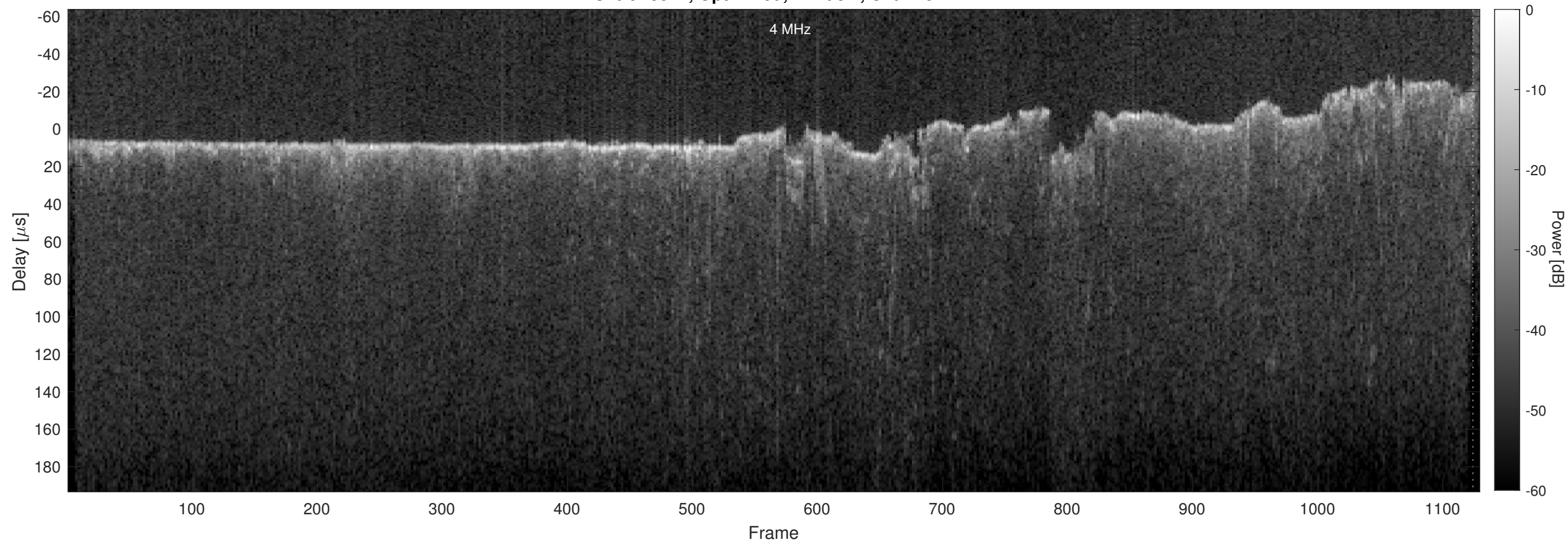
Orbit 13524, Optimized, Window, Channel 2
