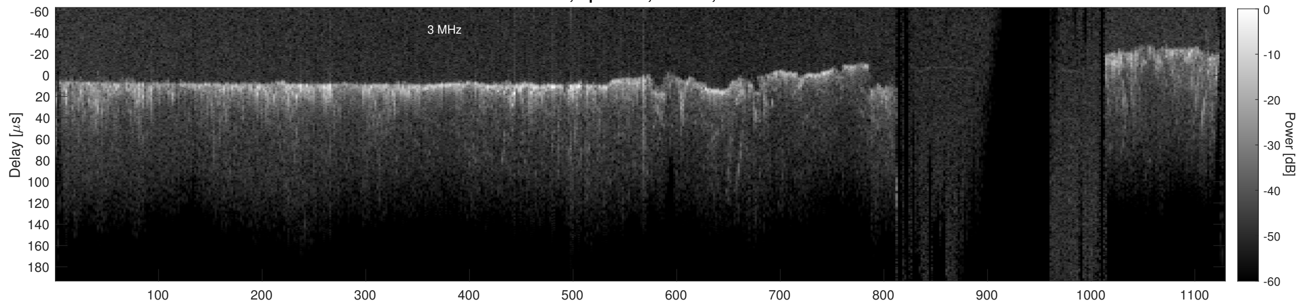
Orbit 13524, Cluttergram
