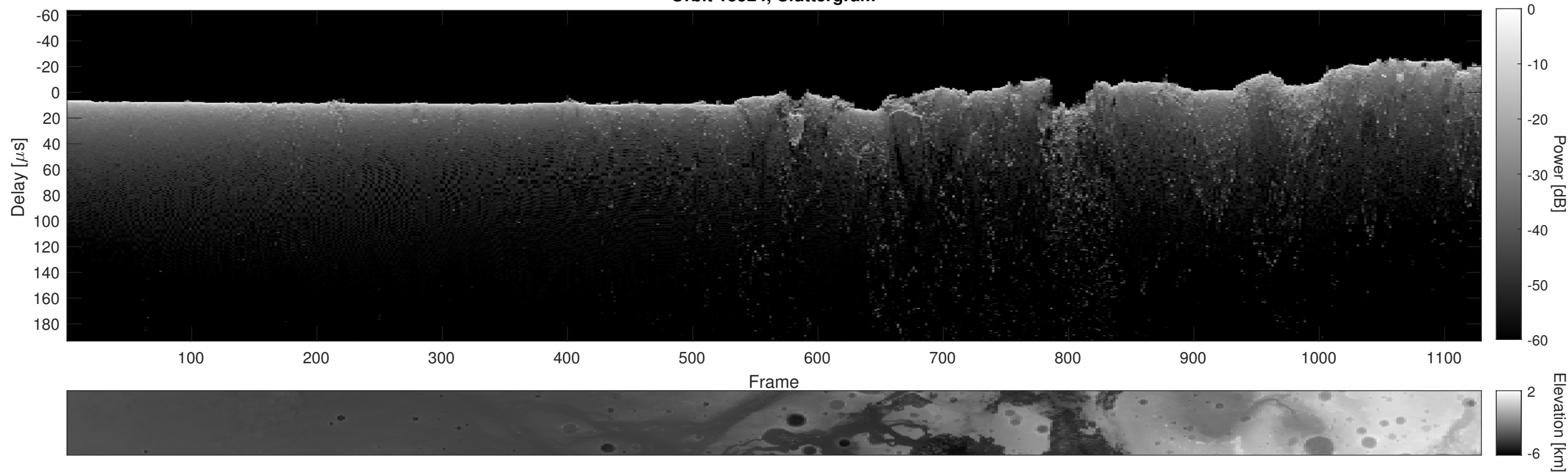
Orbit 13524, Cluttergram
