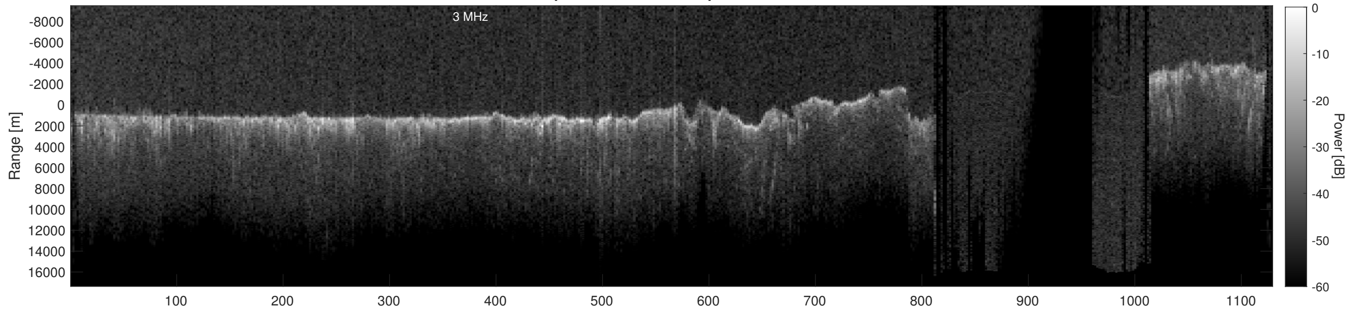
Orbit 13524, Depth-Corrected Cluttergram
