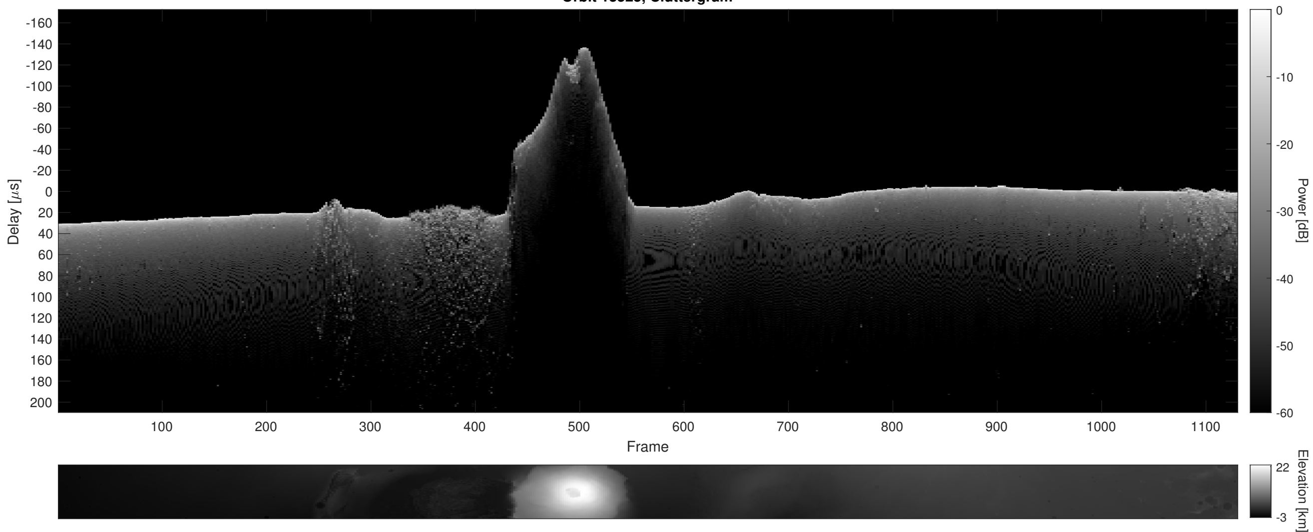
Orbit 13525, Cluttergram
