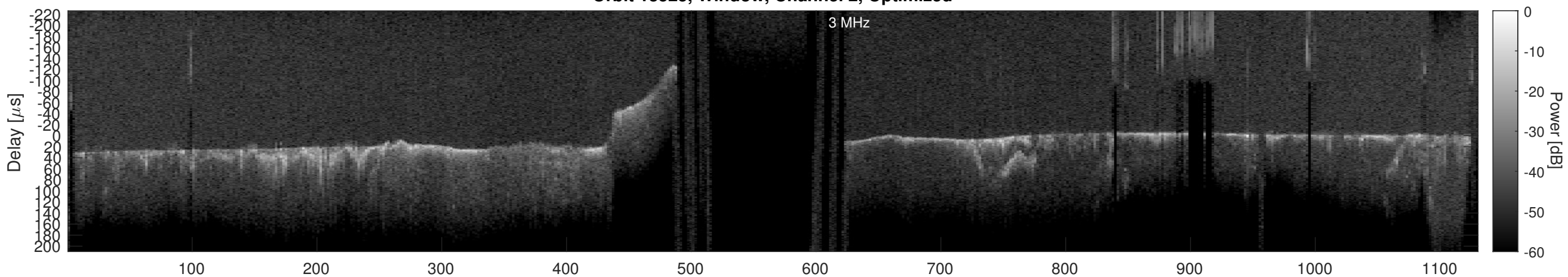
Orbit 13525, Cluttergram
