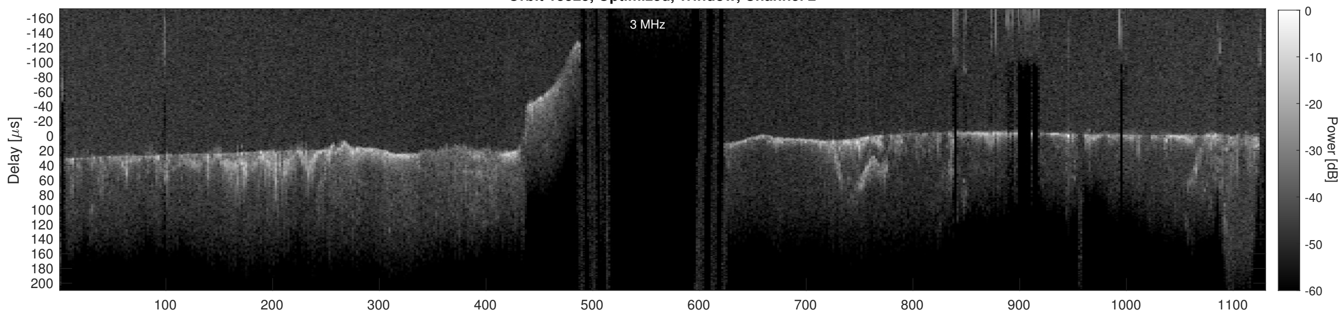
Orbit 13525, Cluttergram
