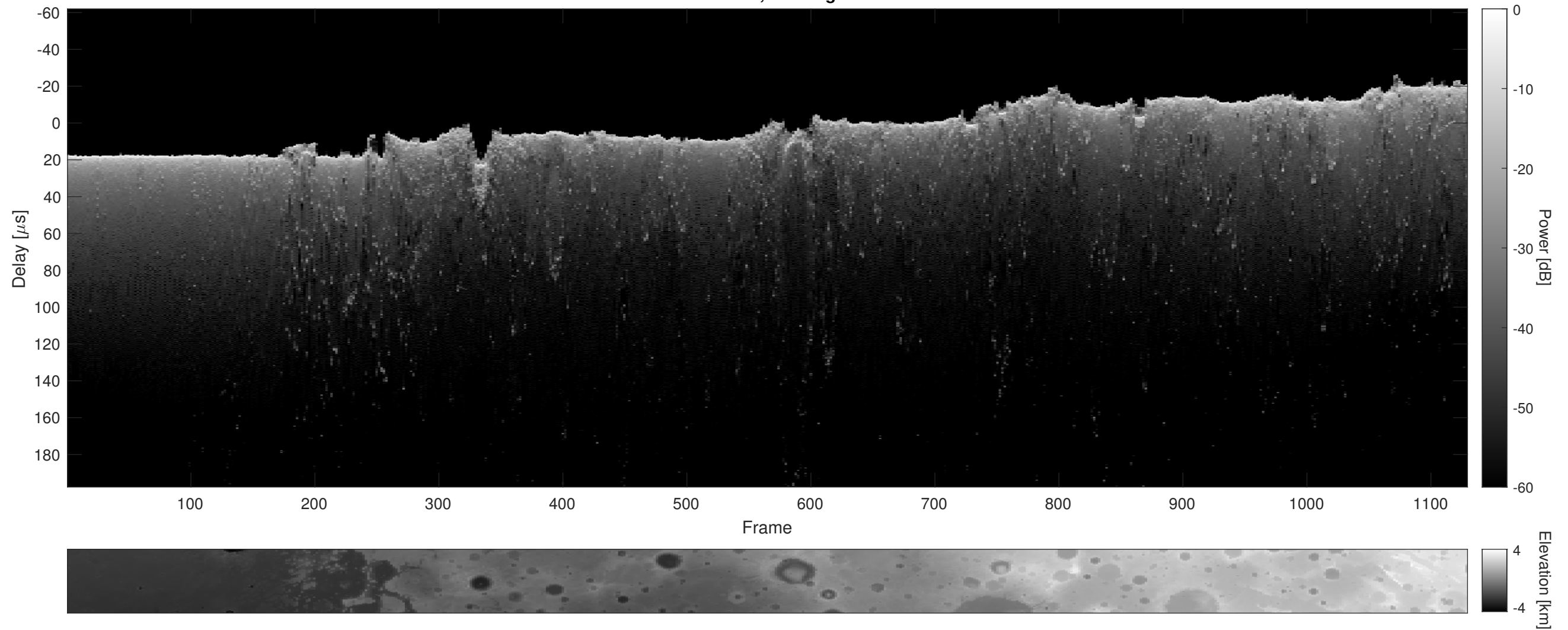
Orbit 13527, Cluttergram
