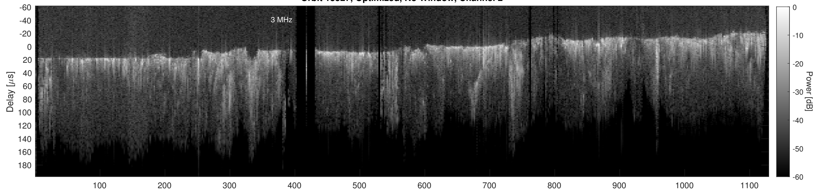
Orbit 13527, Cluttergram
