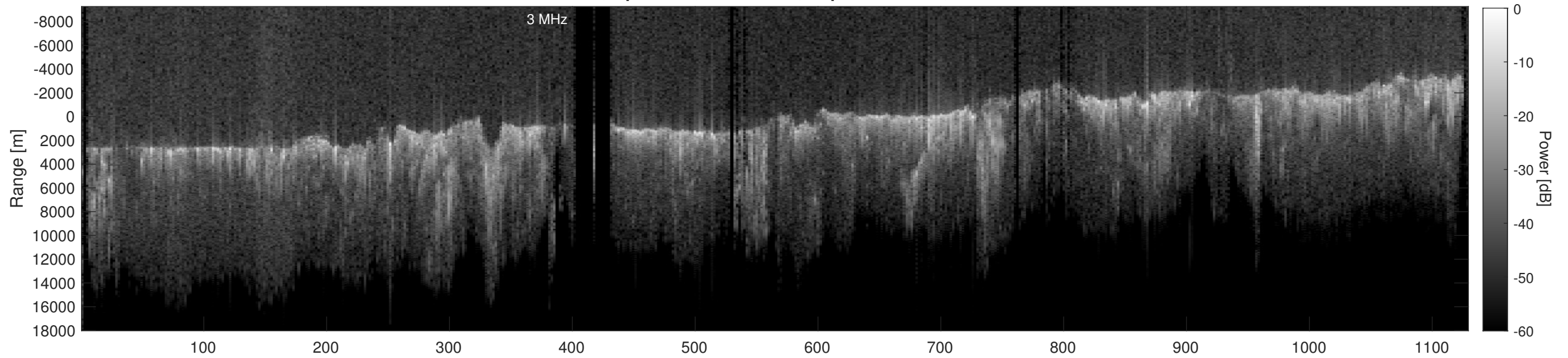
Orbit 13527, Depth-Corrected Cluttergram
