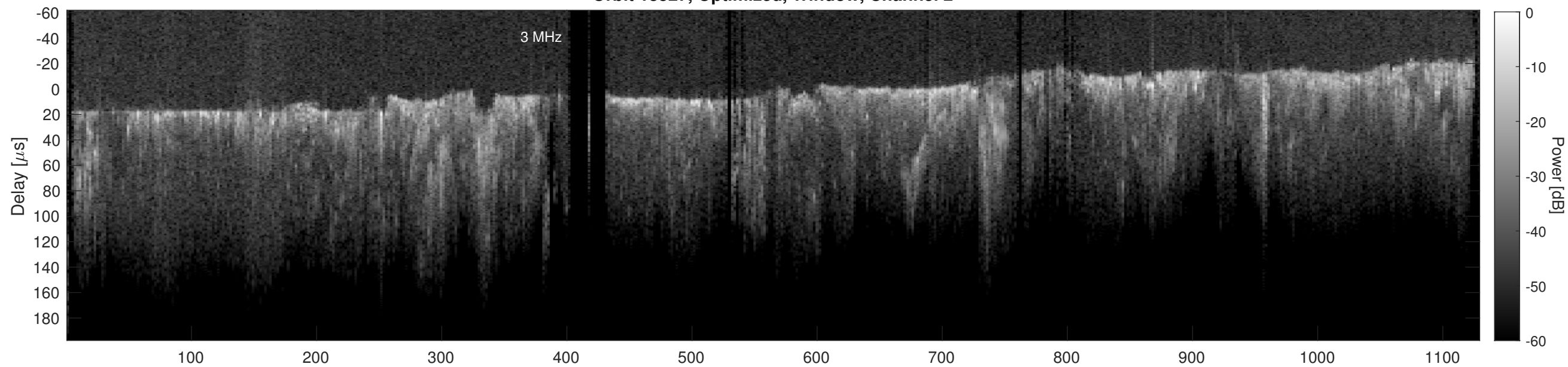
Orbit 13527, Cluttergram
