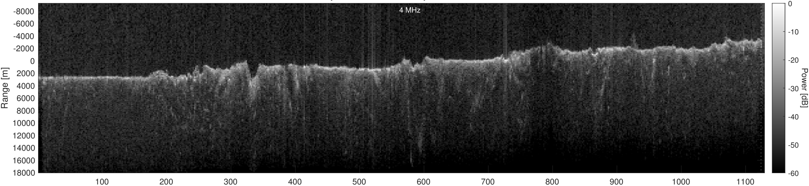
Orbit 13527, Optimized, Window, Depth-Corrected, Channel 2
