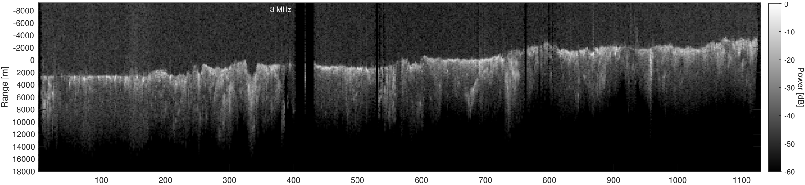
Orbit 13527, Depth-Corrected Cluttergram
