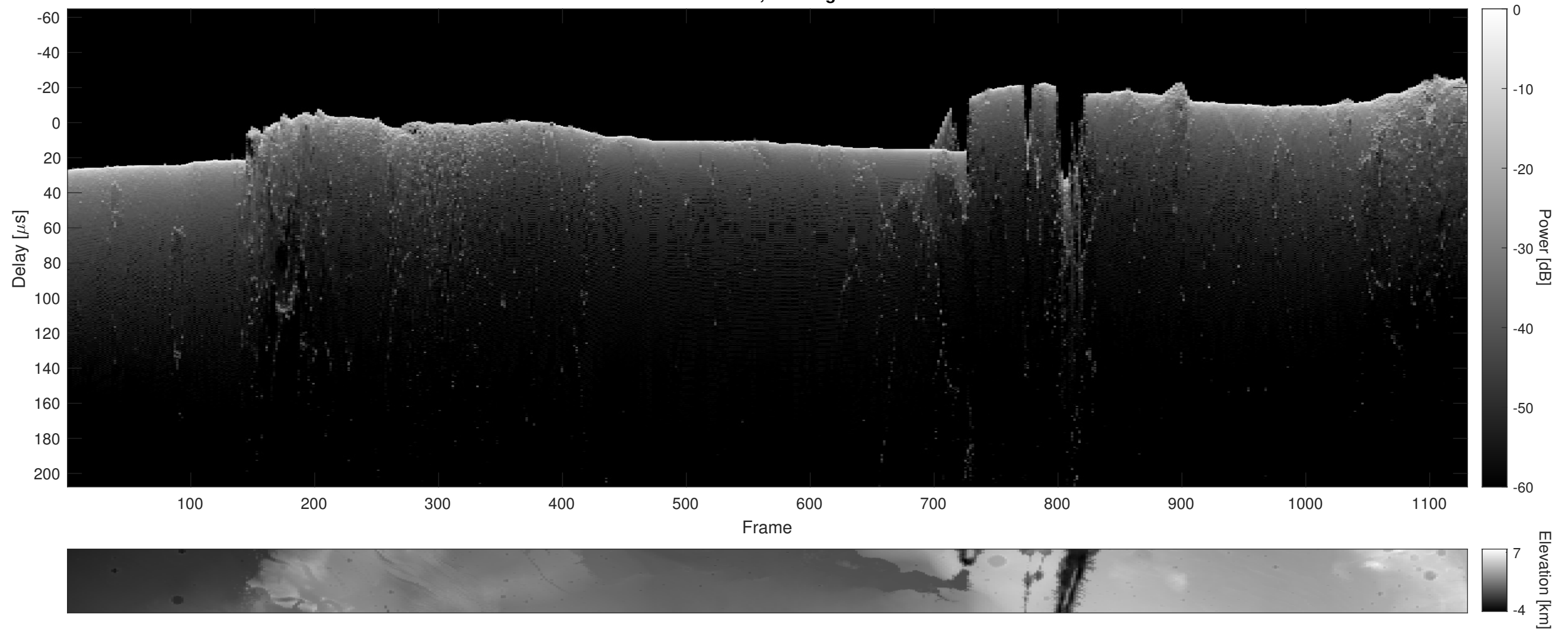
Orbit 13528, Cluttergram
