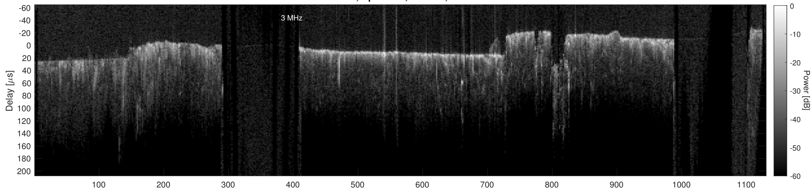
Orbit 13528, Cluttergram
