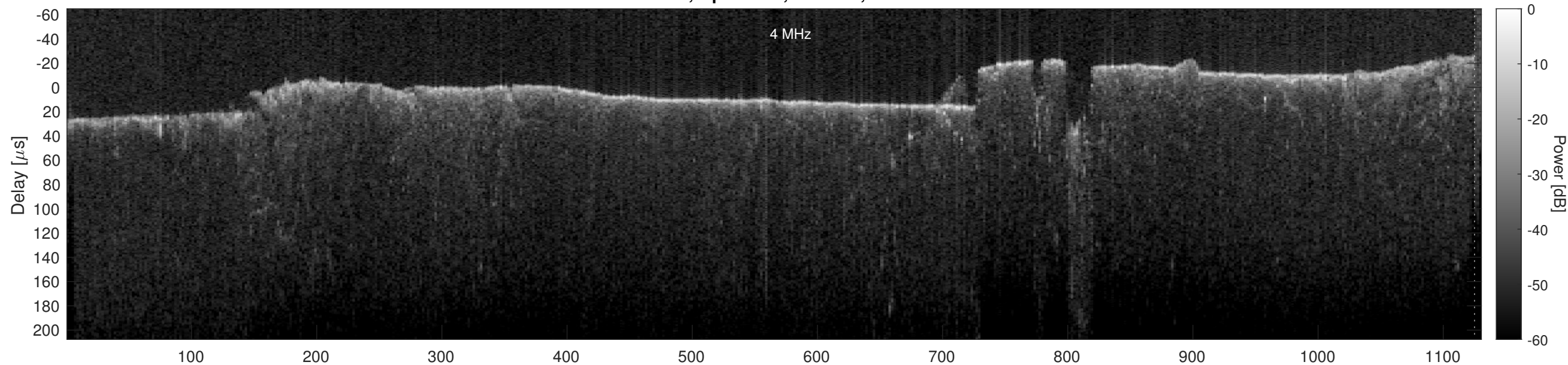
Orbit 13528, Optimized, Window, Channel 2
