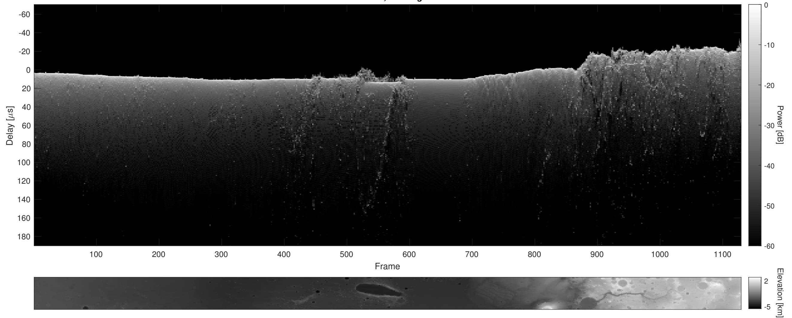
Orbit 13529, Cluttergram
