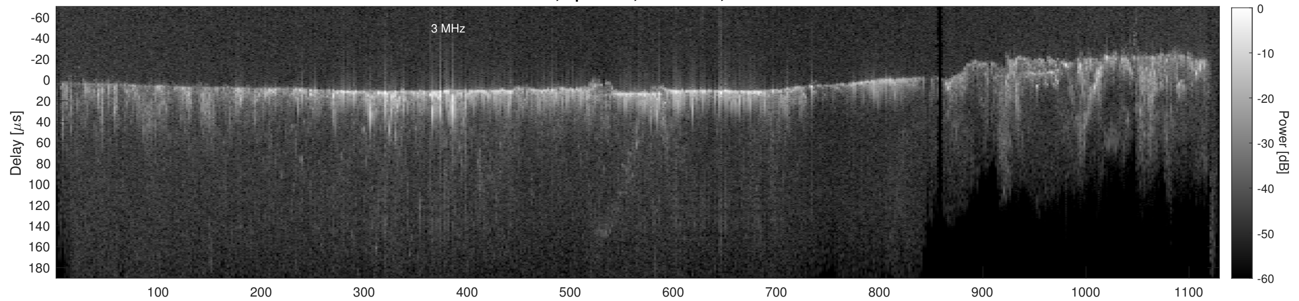
Orbit 13529, Cluttergram
