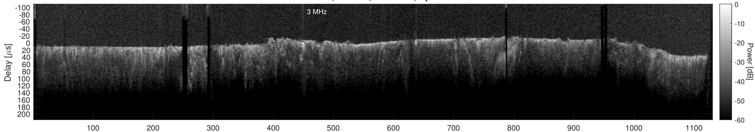
Orbit 13530, Cluttergram
