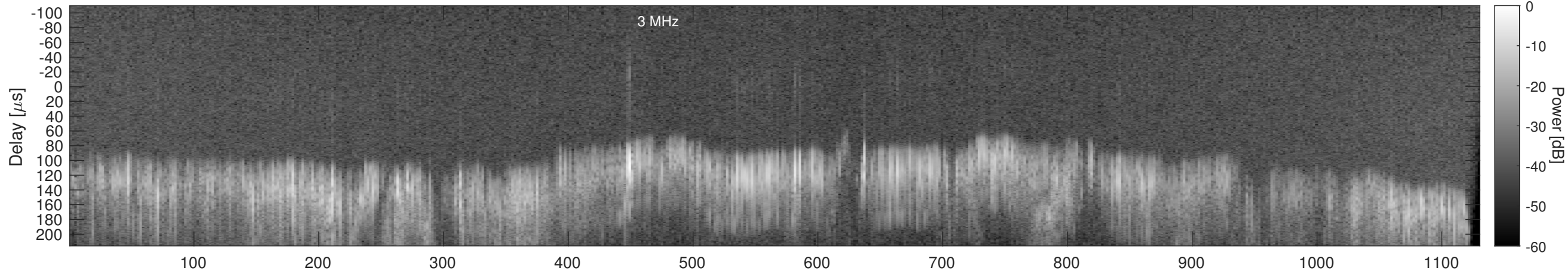
Orbit 13530, Window, Channel 2, Chapman
