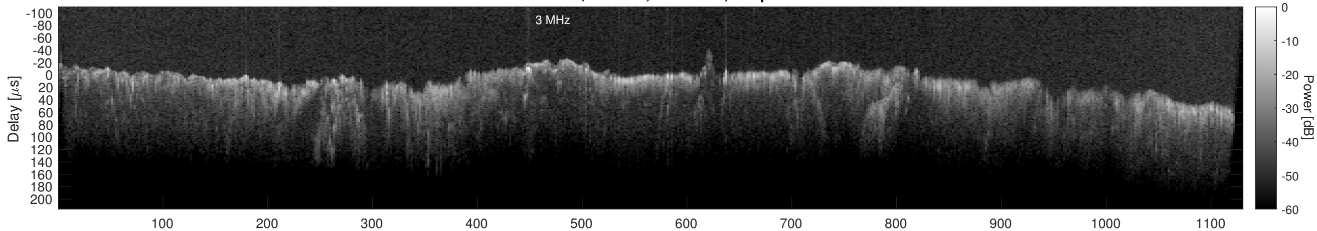
Orbit 13530, Window, Channel 2, Optimized
