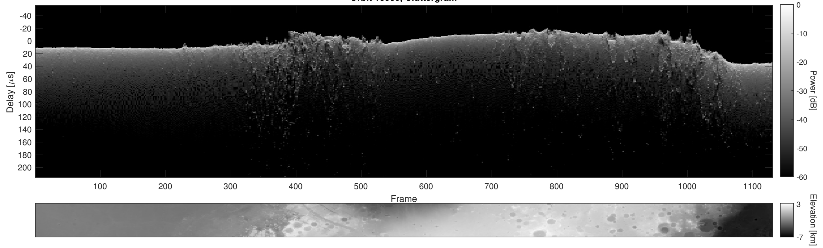
Orbit 13530, Cluttergram
