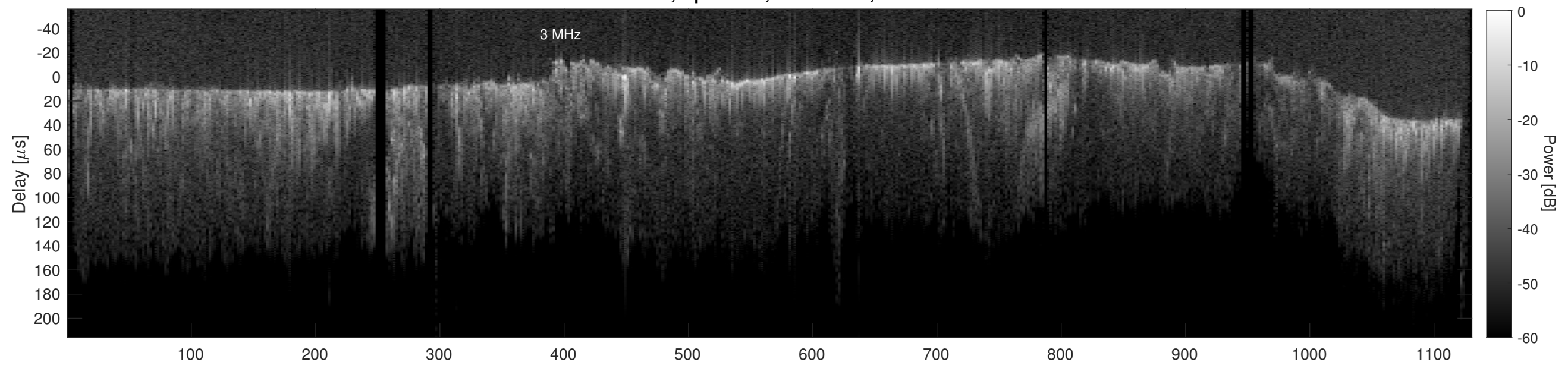
Orbit 13530, Cluttergram
