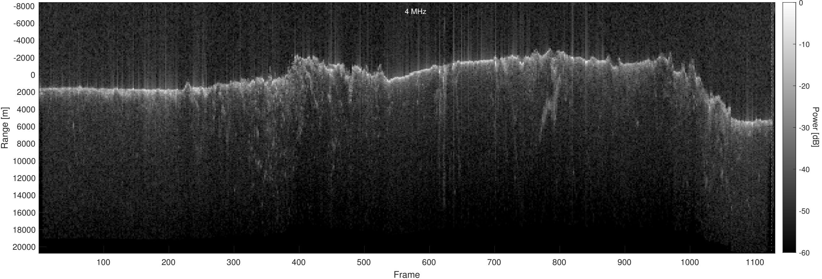
Orbit 13530, Optimized, No Window, Depth-Corrected, Channel 2
