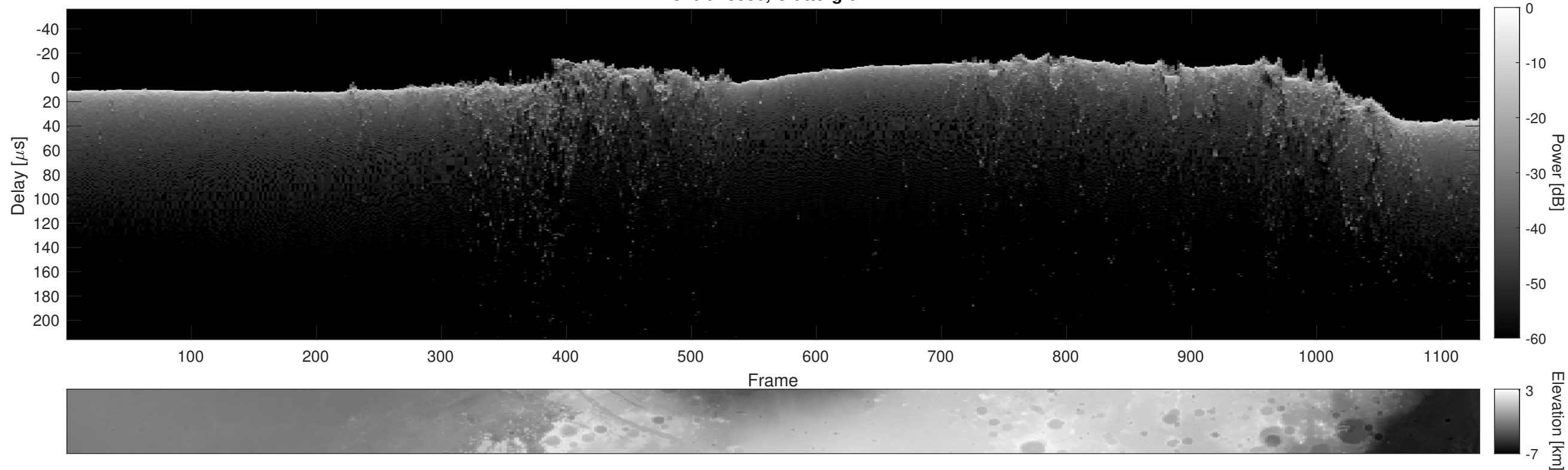
Orbit 13530, Cluttergram
