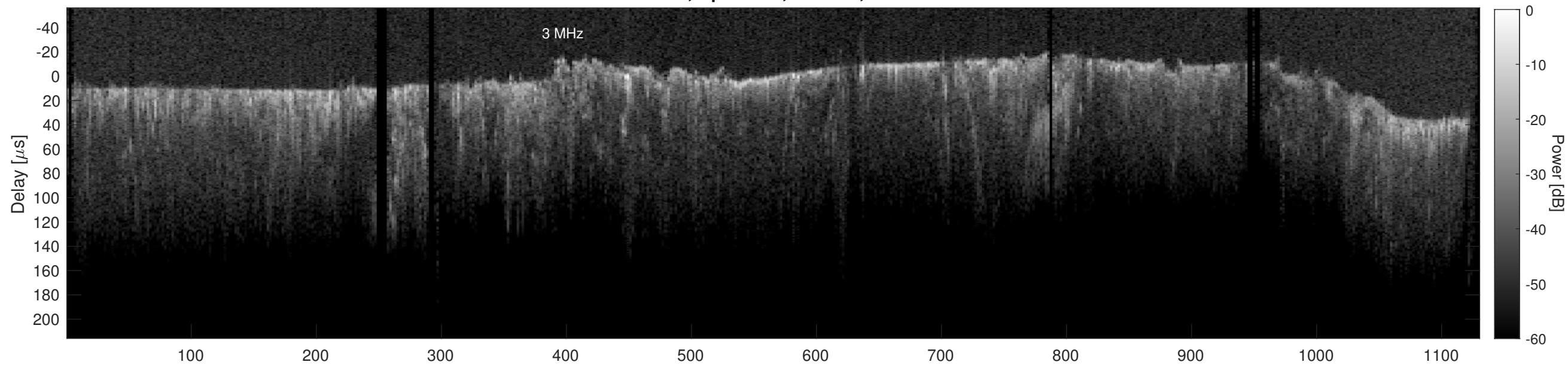
Orbit 13530, Cluttergram
