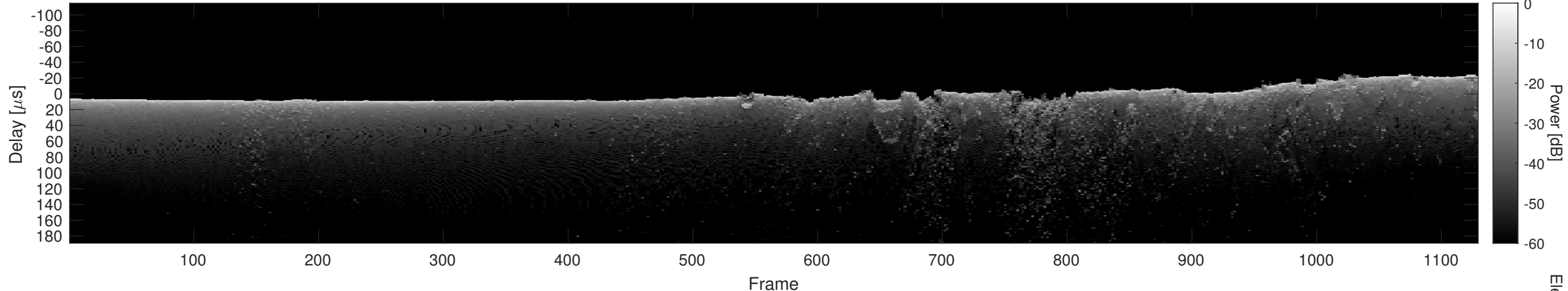
Orbit 13531, Cluttergram
