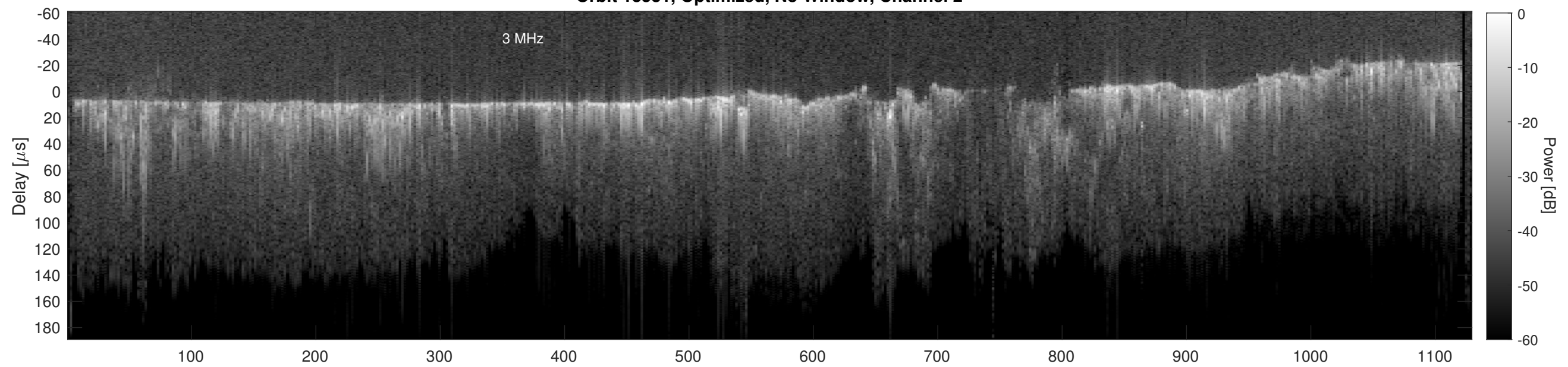
Orbit 13531, Cluttergram
