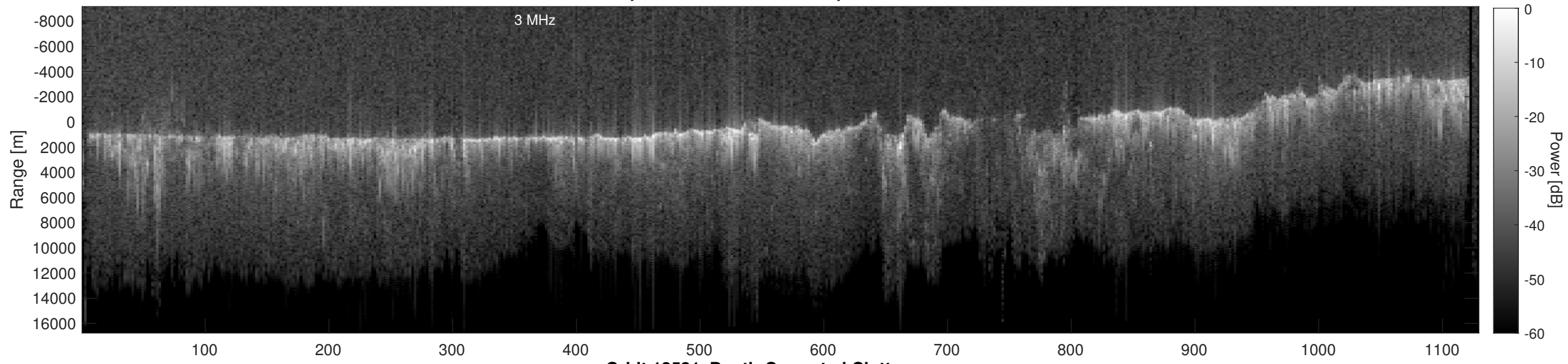
Orbit 13531, Depth-Corrected Cluttergram
