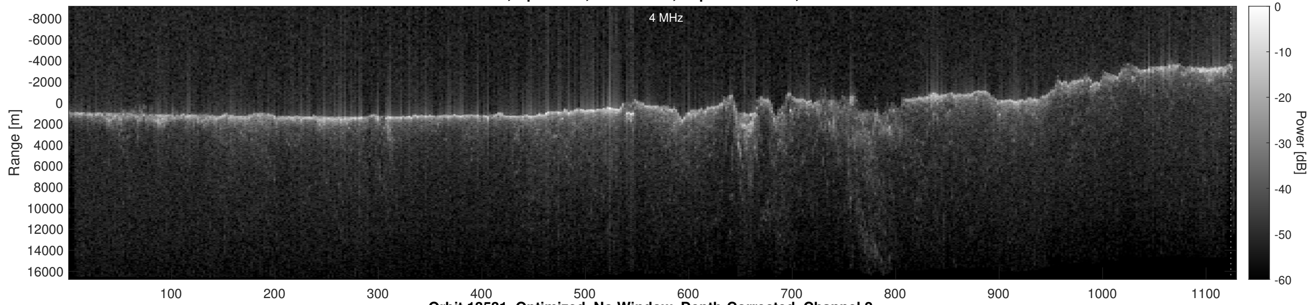
Orbit 13531, Optimized, No Window, Depth-Corrected, Channel 2
