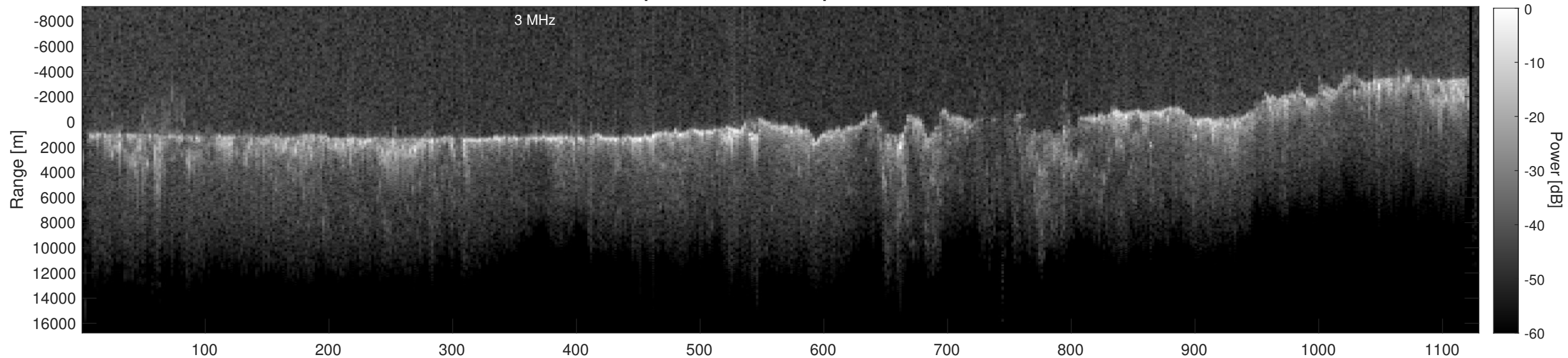
Orbit 13531, Depth-Corrected Cluttergram
