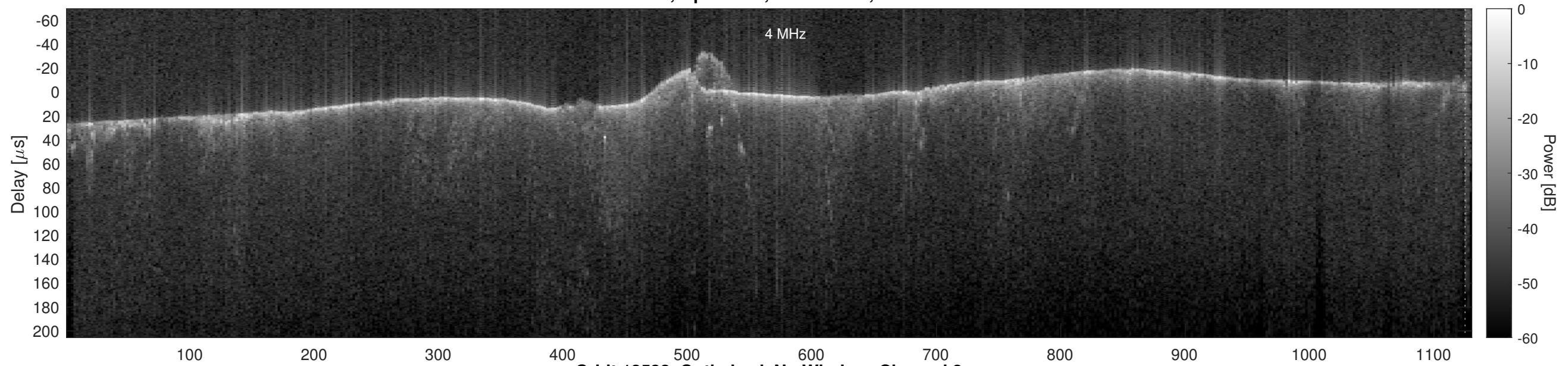
Orbit 13532, Optimized, No Window, Channel 2
