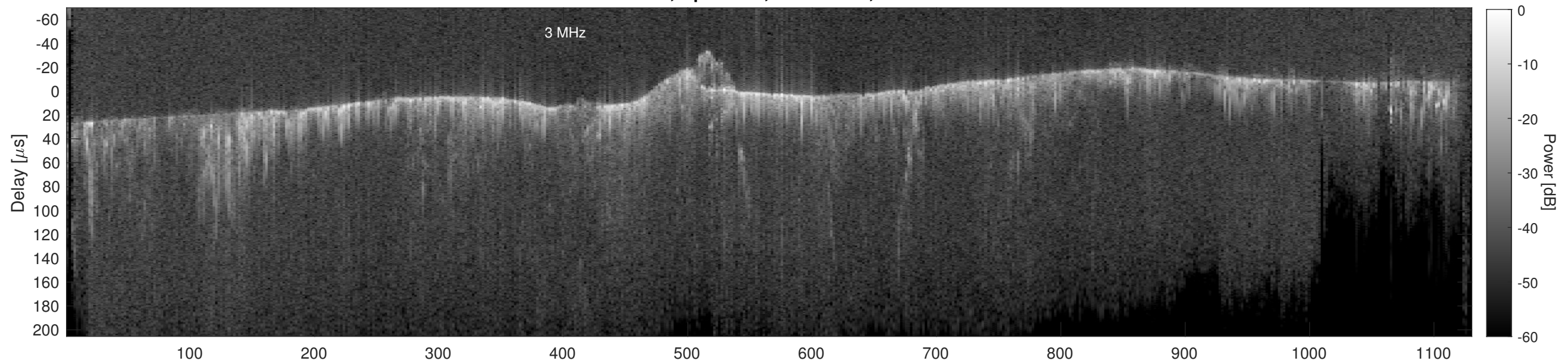
Orbit 13532, Cluttergram
