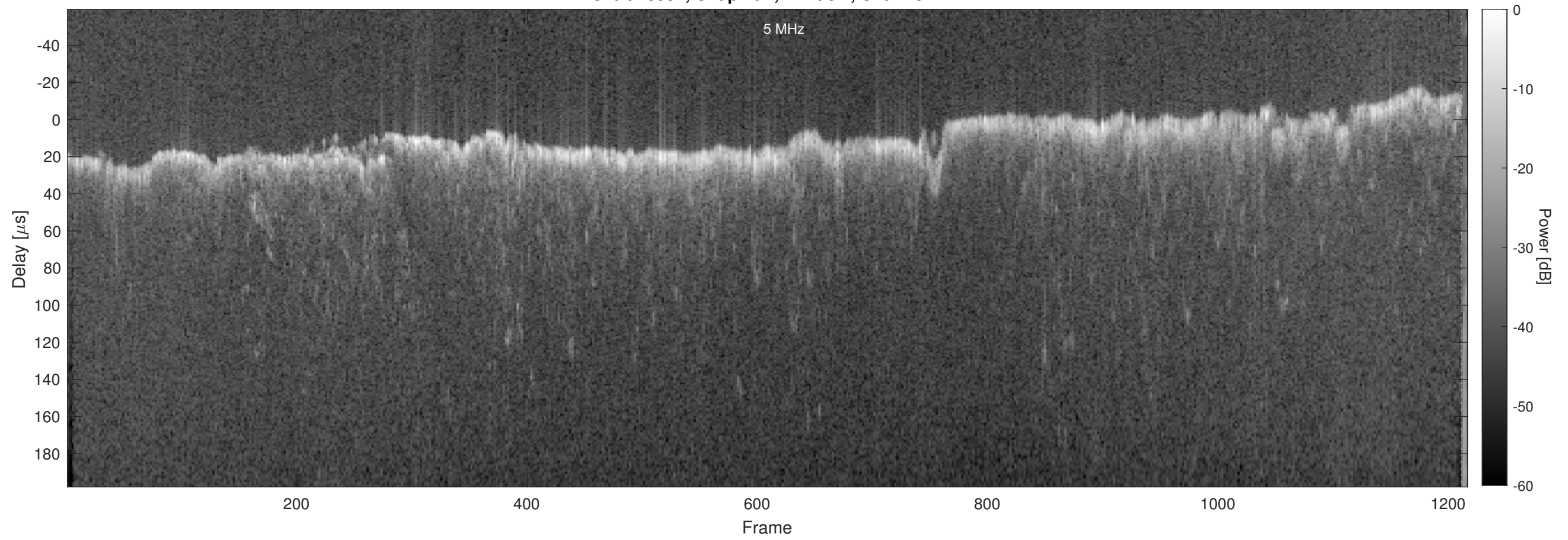
Orbit 13534, Chapman, Window, Channel 2
