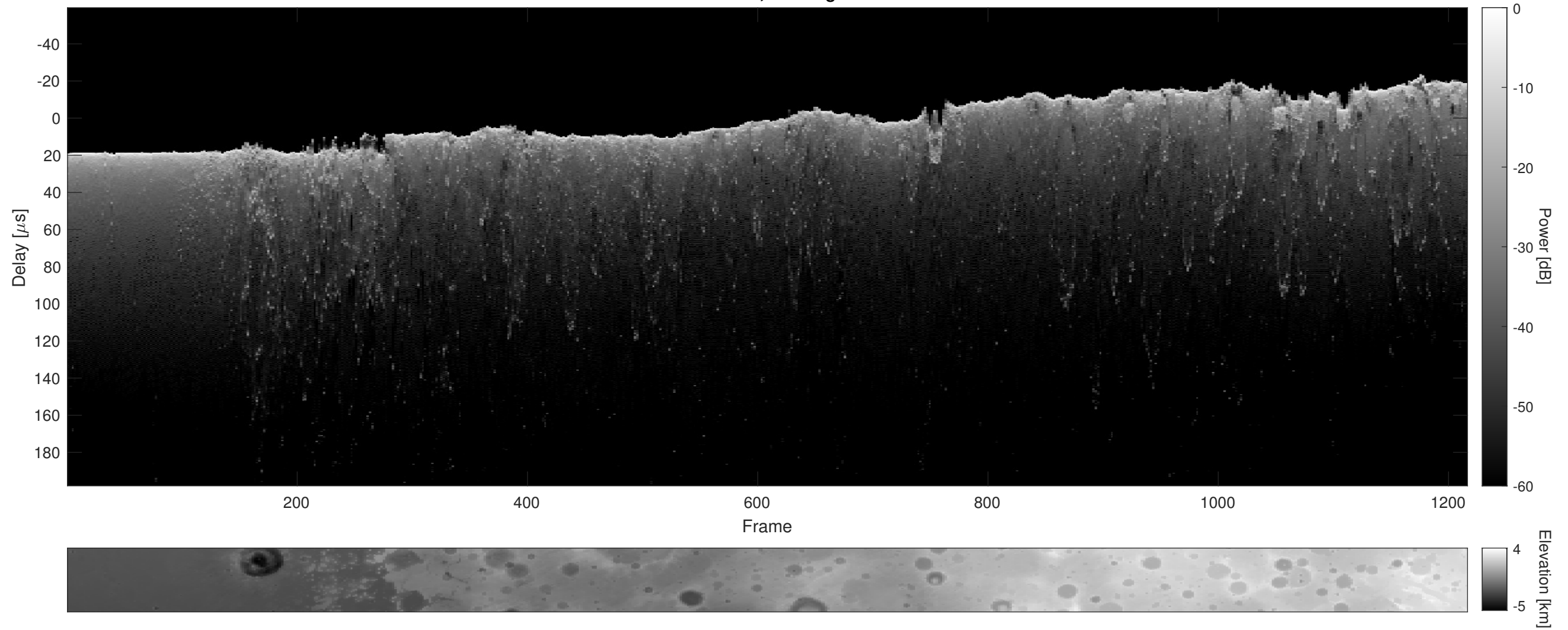
Orbit 13534, Cluttergram
