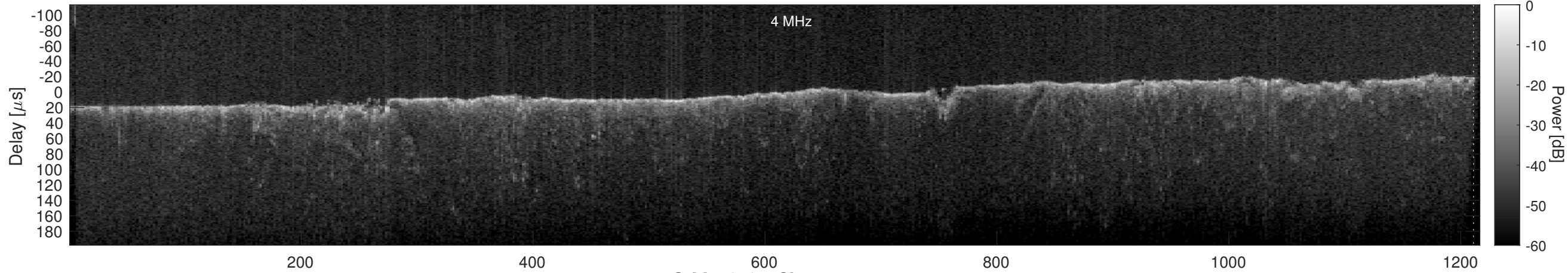
Orbit 13534, Cluttergram
