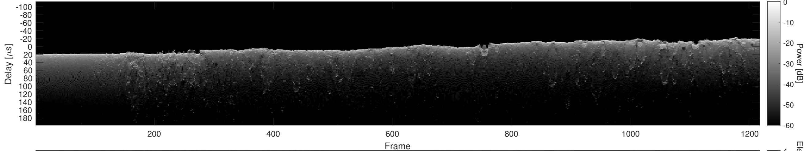
Orbit 13534, Cluttergram
