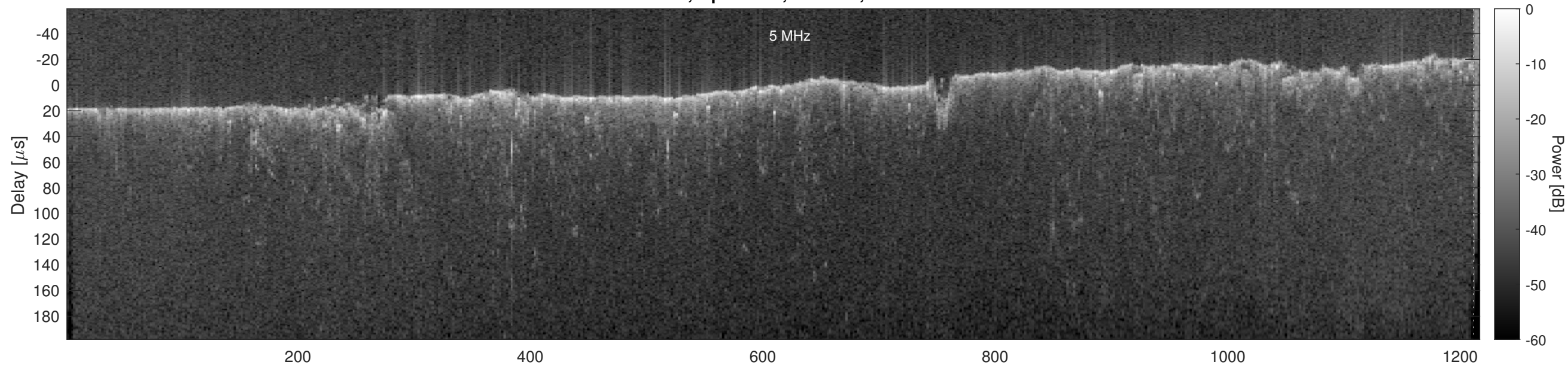
Orbit 13534, Optimized, Window, Channel 2
