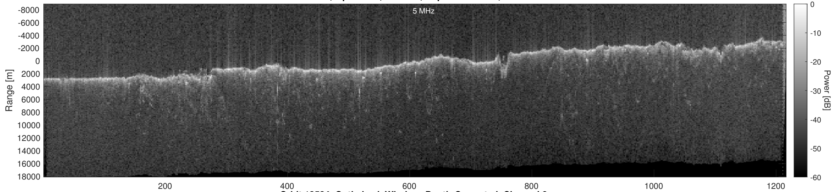
Orbit 13534, Optimized, Window, Depth-Corrected, Channel 2
