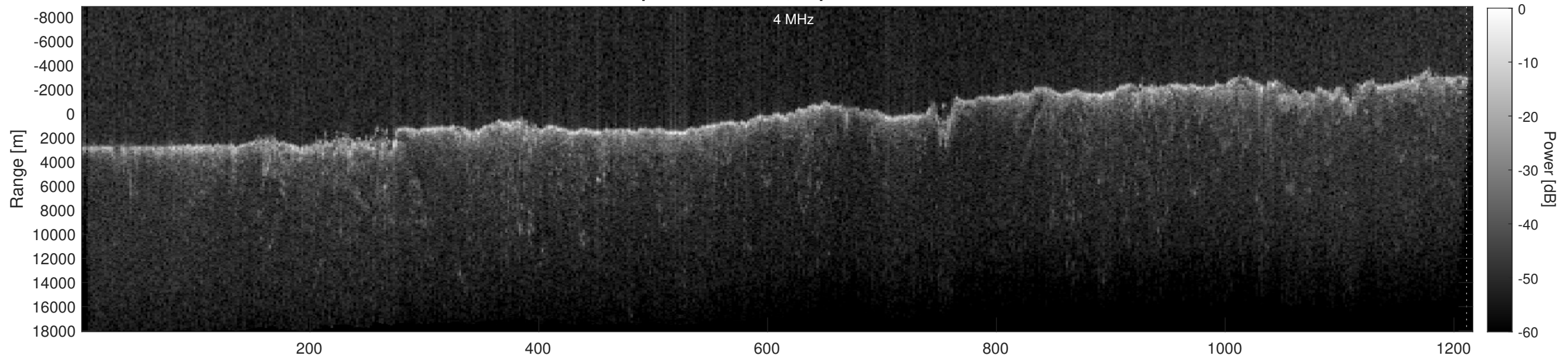
Orbit 13534, Depth-Corrected Cluttergram
