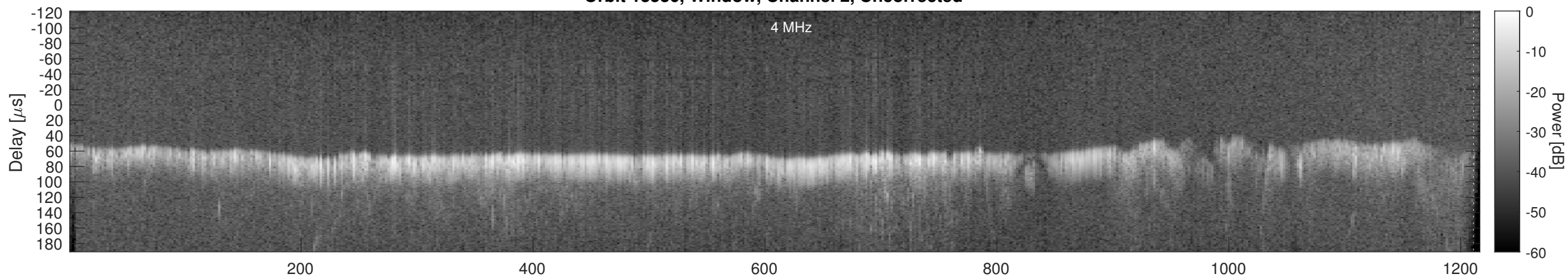
Orbit 13536, Window, Channel 2, Chapman
