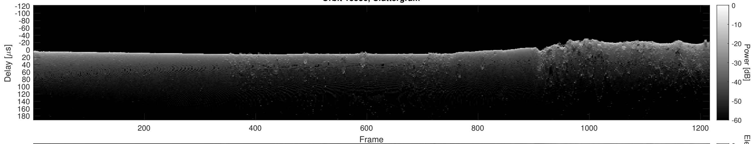
Orbit 13536, Cluttergram
