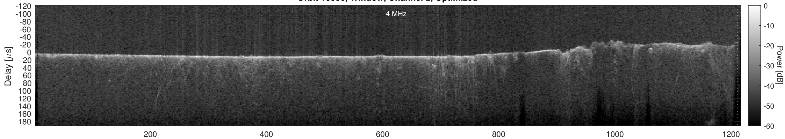
Orbit 13536, Cluttergram
