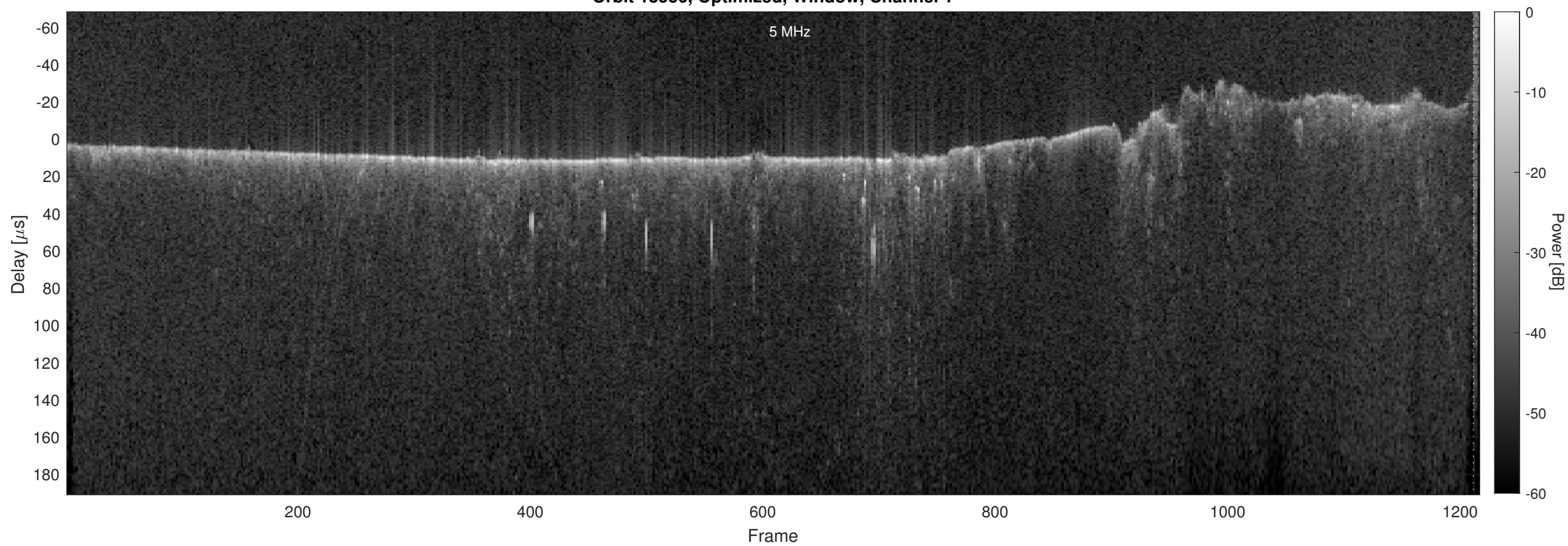
Orbit 13536, Optimized, Window, Channel 2
