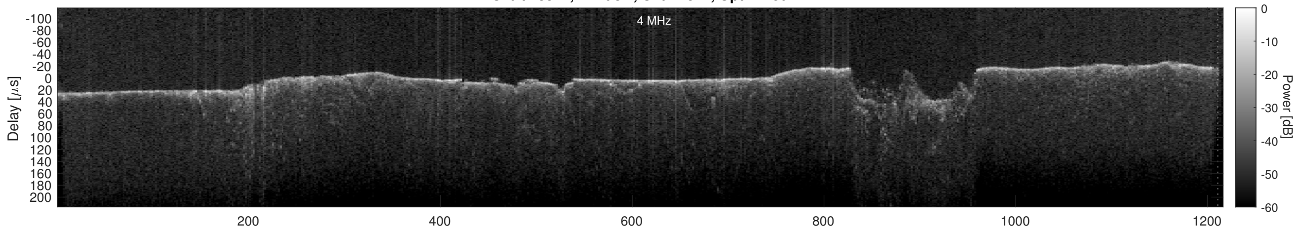
Orbit 13542, Cluttergram
