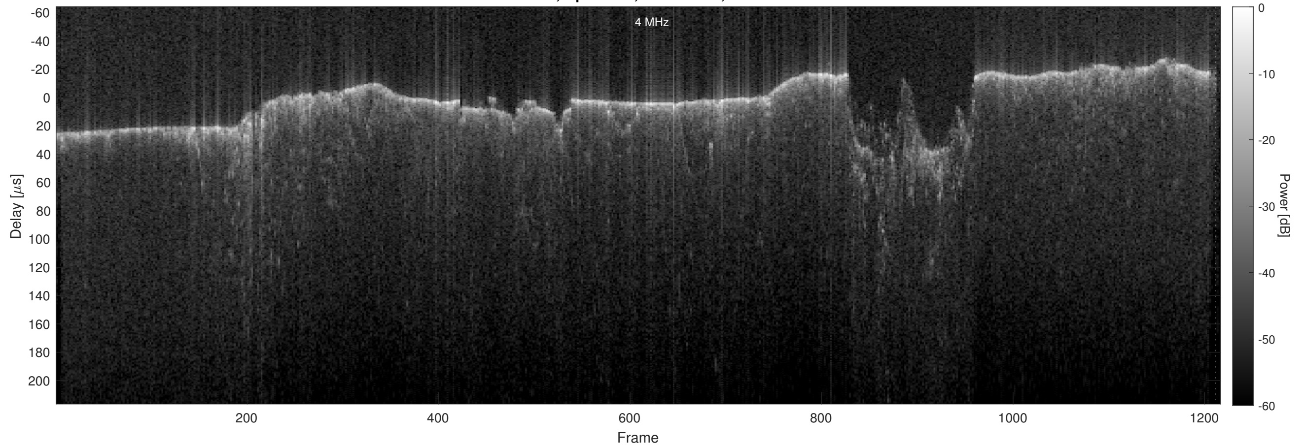
Orbit 13542, Optimized, No Window, Channel 2
