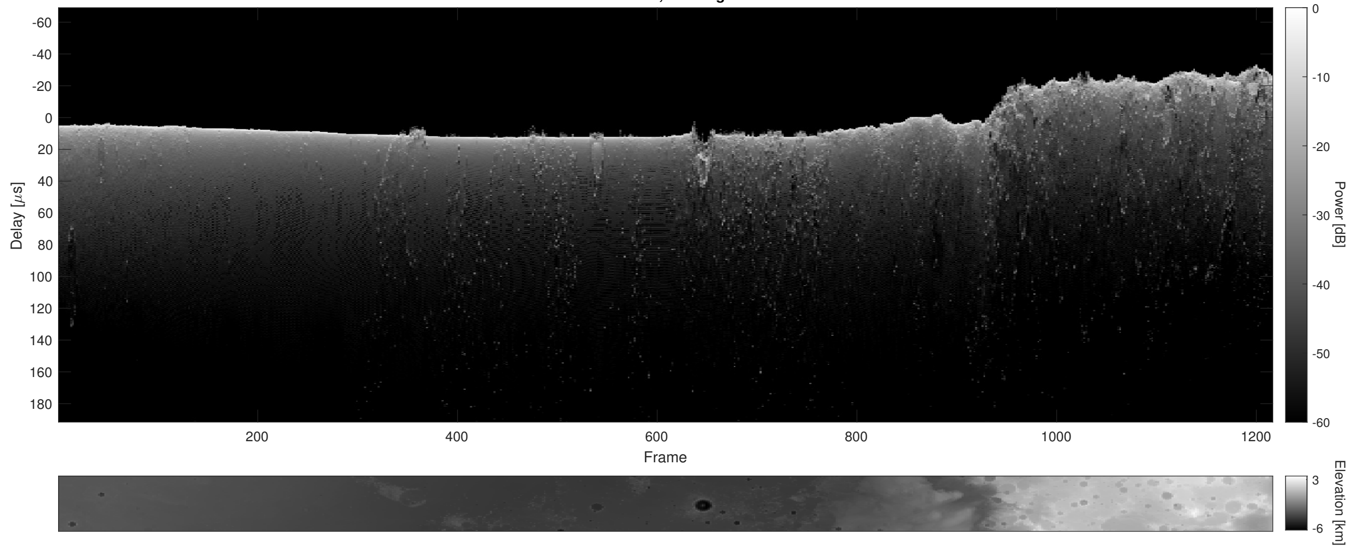
Orbit 13543, Cluttergram
